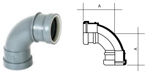
Swept Bend 87.5°
