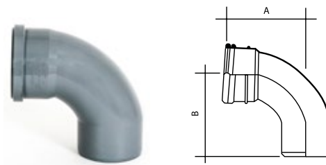
Bends 87.5°
