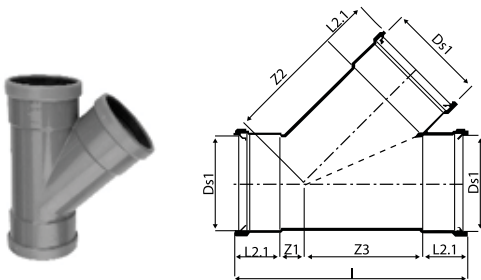
45° Y (Tee) Branch (3 Socket)
