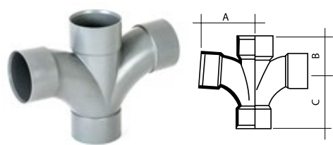
Cross Tee 87.5°
