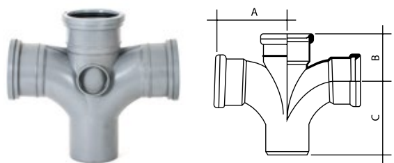
Cross Tee 87.5°
