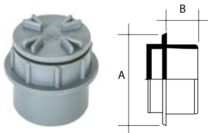
Access Plug (With Screw Cap)
