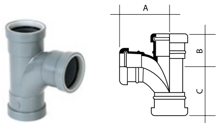
Swept Tee 87.5°
