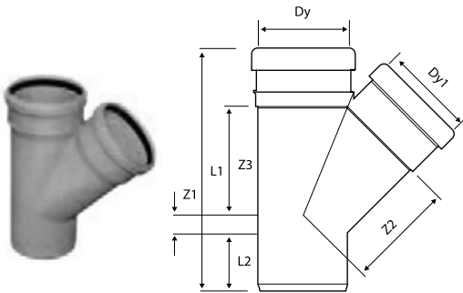
45° Y (Tee) Branch (2 Socket / Spigot )
