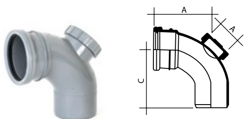
Access Bend 87.5°
