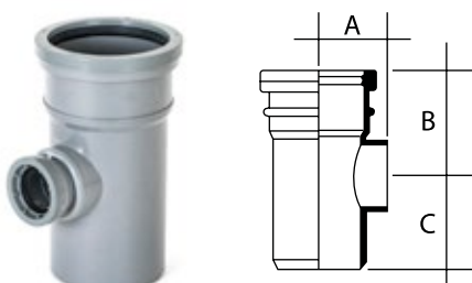
Branch Unequal 87.5° (Bossed Pipe)
