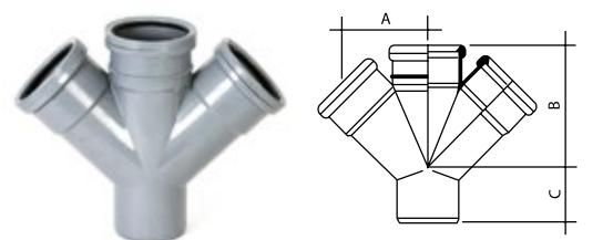
Double Branch 45°
