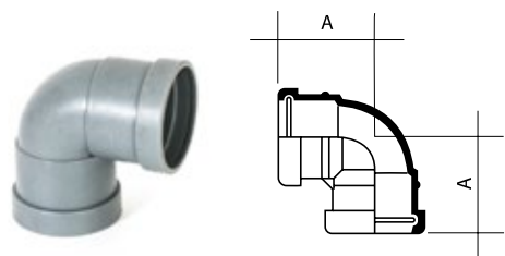
Knuckle Bend 90°
