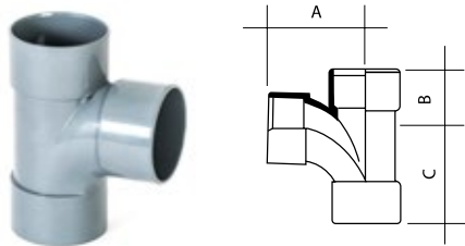
Swept Tee 92.50° (Triple Socket)
