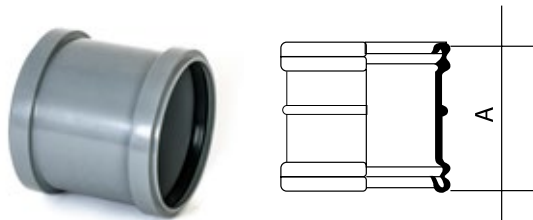
Double Socket Coupler
